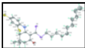
Fig. 1. Anisotropic displacement ellipsoid plot (Barbour, 2001) plot of C_{26}H_{37}Cl_2NOS_2 at the 70% probability level; hydrogen atoms are drawn as spheres of arbitrary radius.
